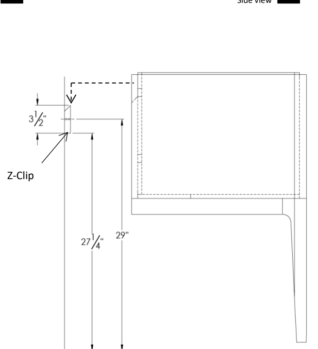
Wall-mounted vanity legs 9 Side view
