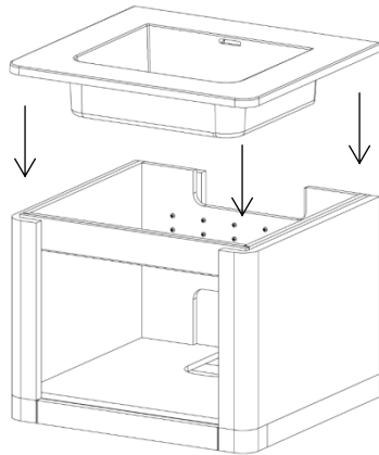
Wall-mounted vanity Perspective view
