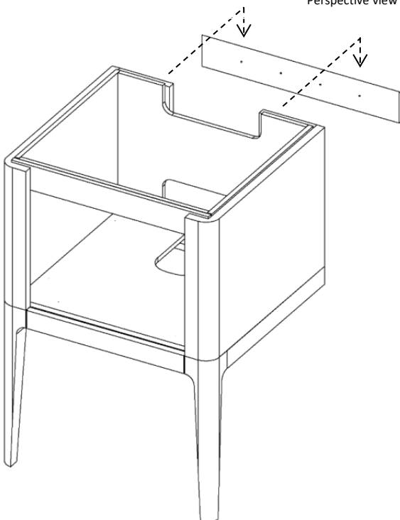
Wall-mounted vanity legs 9 Perspective view
