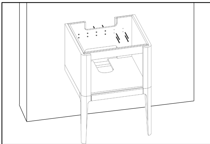
Wall-mounted vanity legs Perspective view 10
