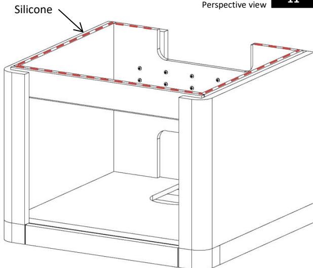
Wall-mounted vanity Perspective view 11
